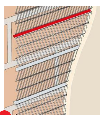
I Carrier for plaster and render finishes
