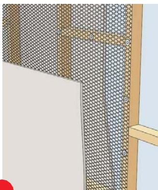
E Security mesh for timber stud walls
