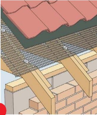
A Security mesh for roofs
